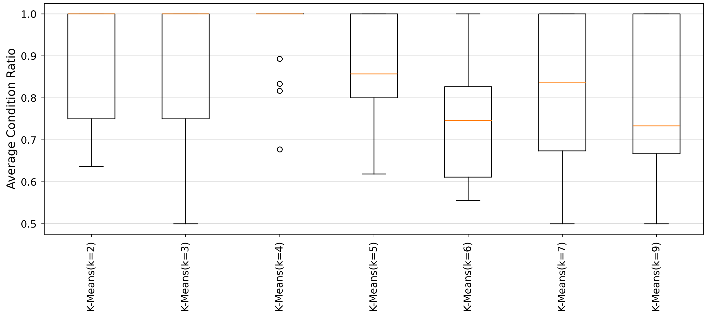
YARA Rules Average Condition Ratio Distribution (Cluster13_Size9 dataset)
